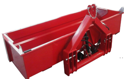
Fig. 2 Pala idraulica HYDRO MIDI con cassone (sponda abbassata) Hydraulic bucket HYDRO MIDI cargo function (lowered front panel)
